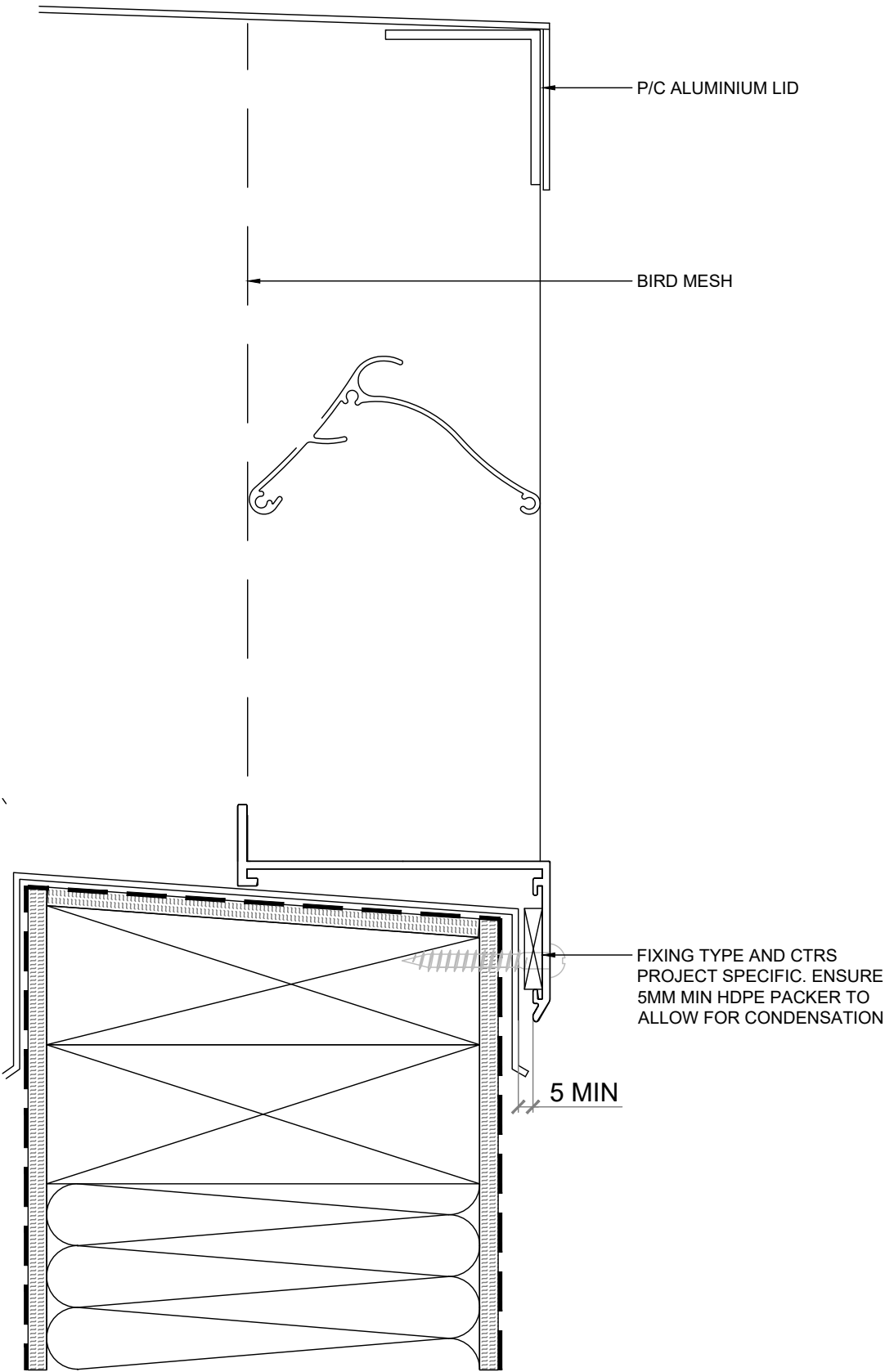
SECTION VIEW
