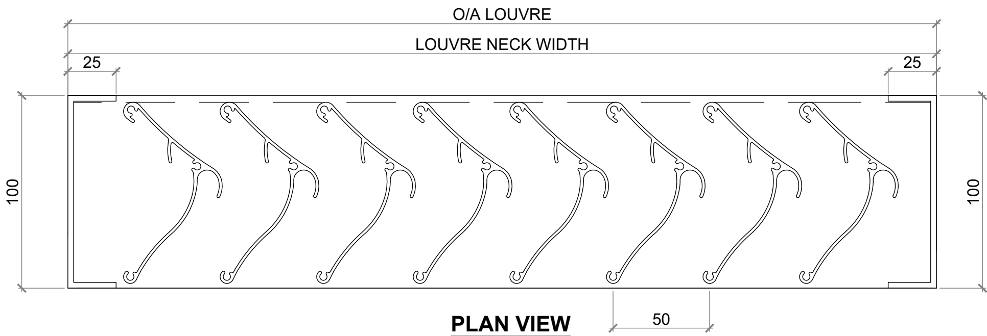
SECTION VIEW
