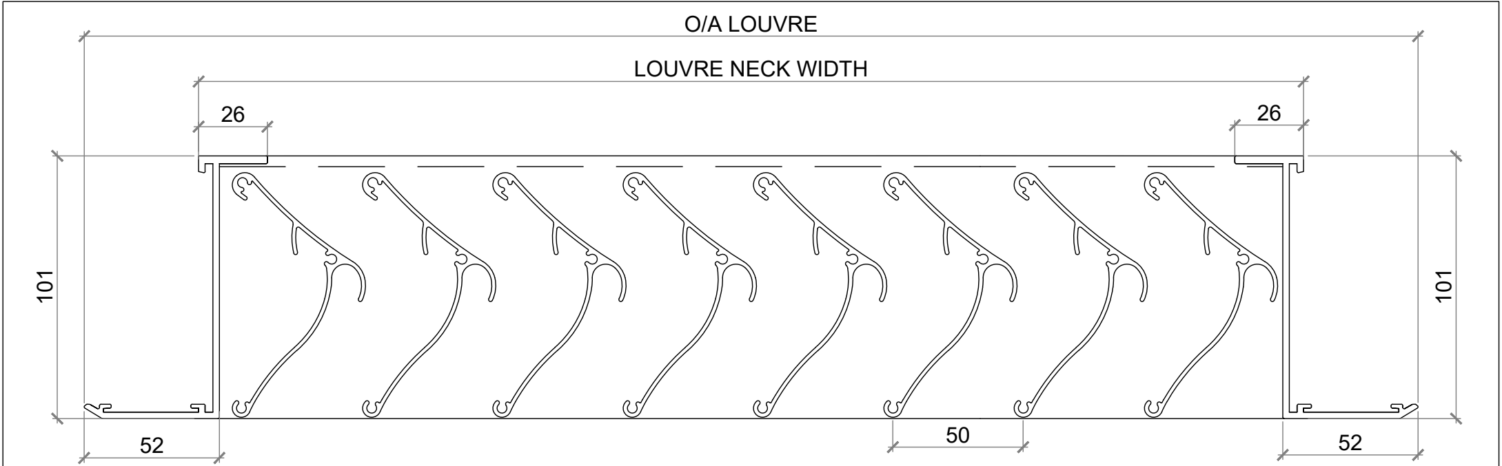
PLAN VIEW
