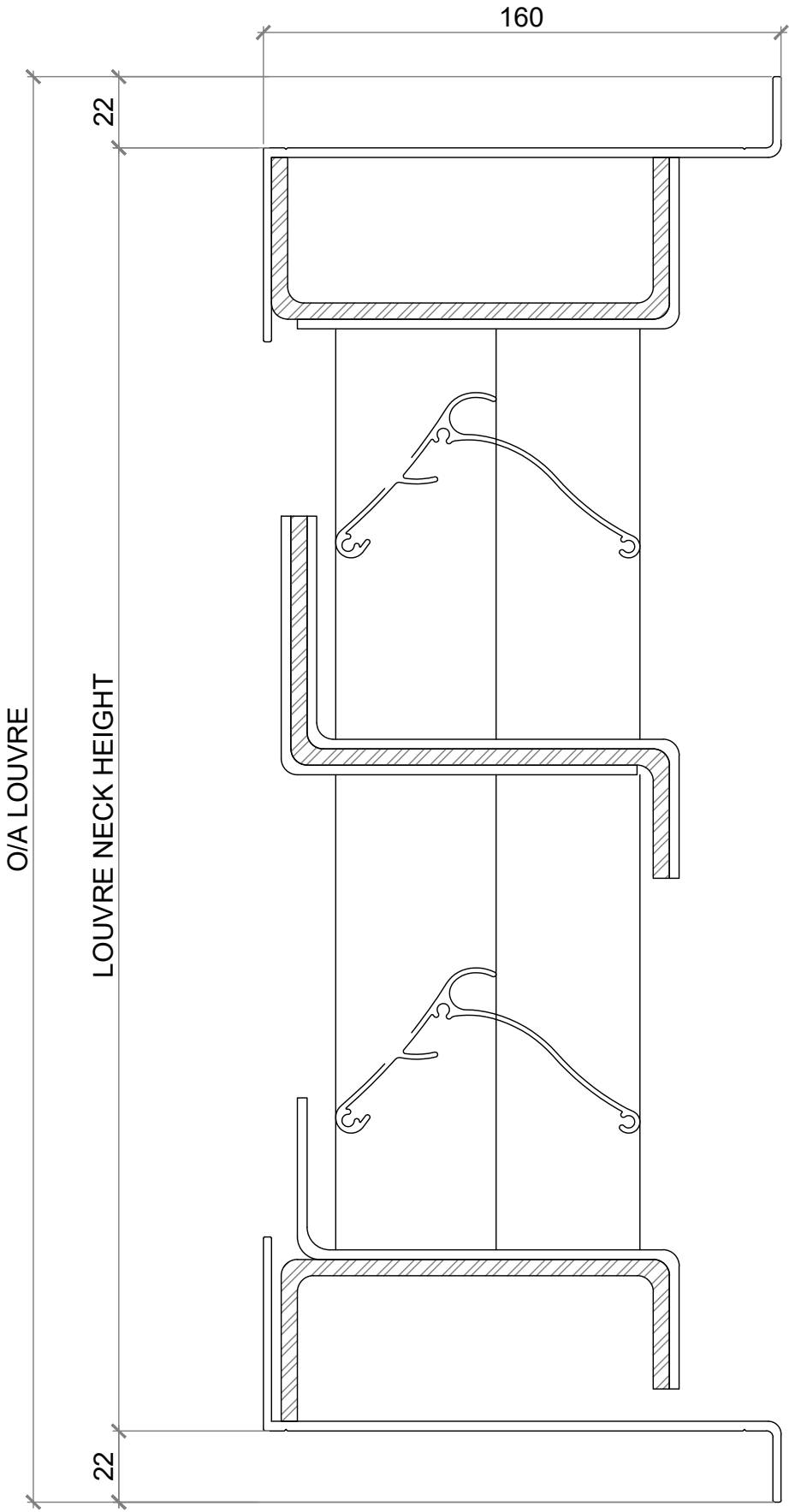
SECTION VIEW
