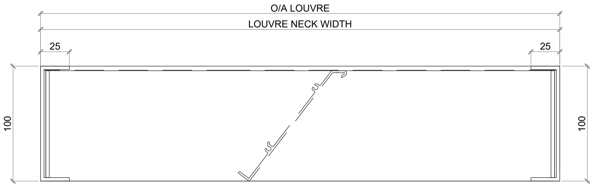
PLAN VIEW
