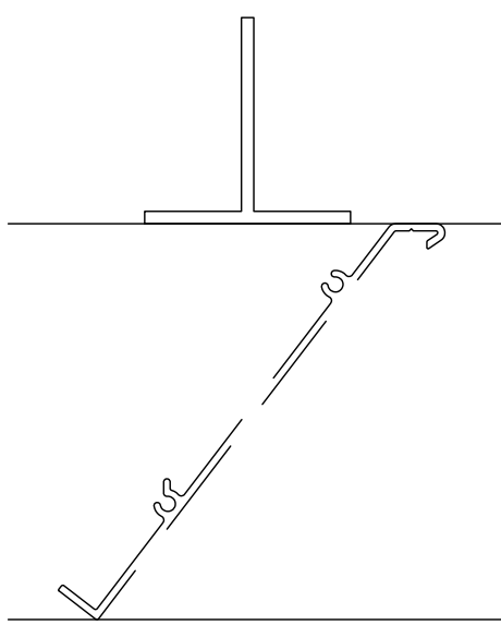
INTERMEDIATE STIFFENER REQUIRED FOR SPECIFIC LOADS
