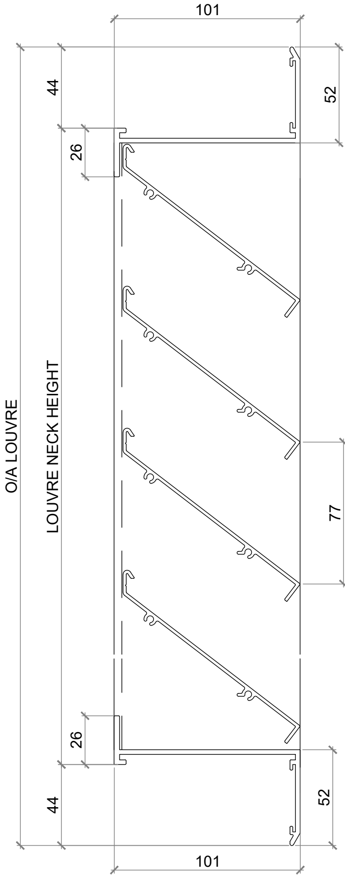
SECTION VIEW
