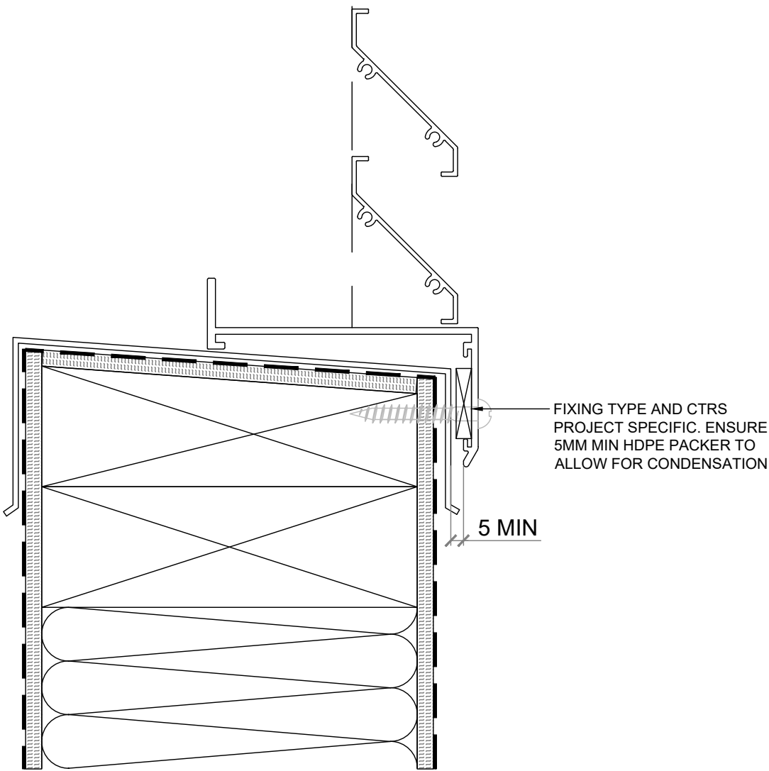
SECTION VIEW
