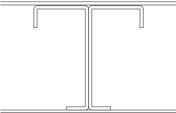
INTERMEDIATE STIFFENER REQUIRED FOR SPECIFIC LOADS
