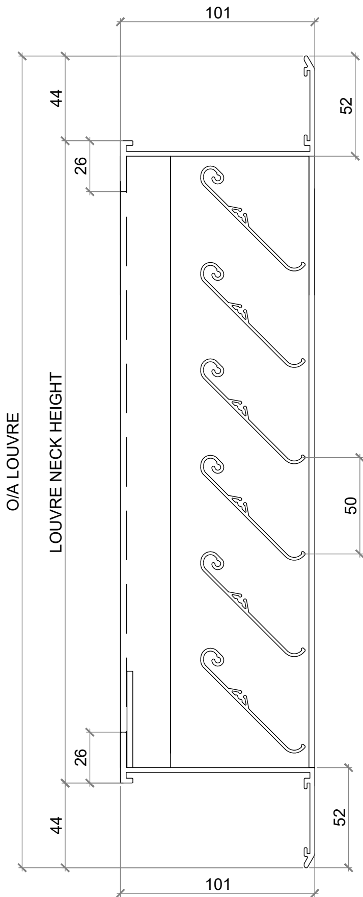
SECTION VIEW
