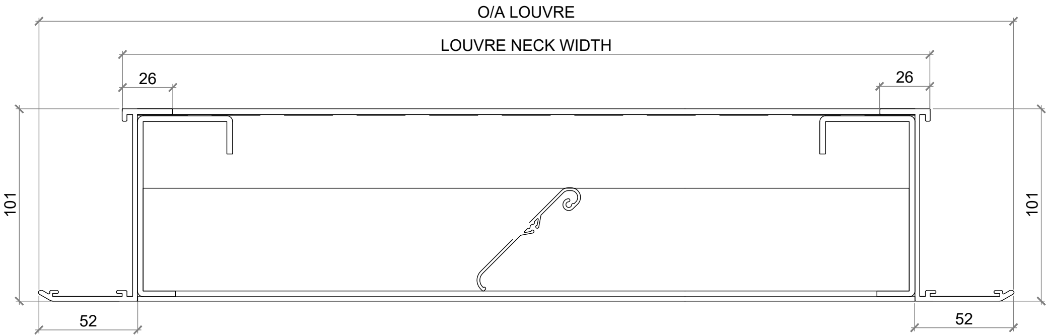
PLAN VIEW
