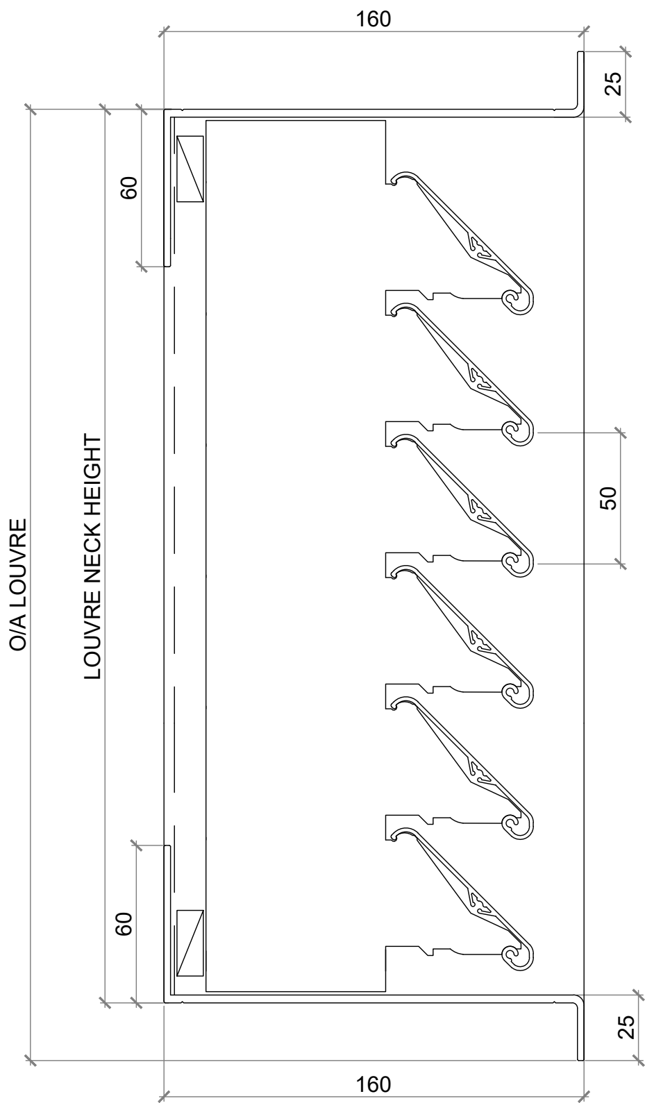
SECTION VIEW
