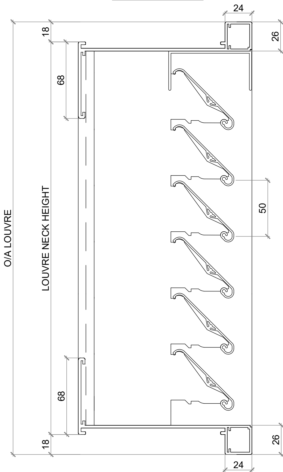
SECTION VIEW
