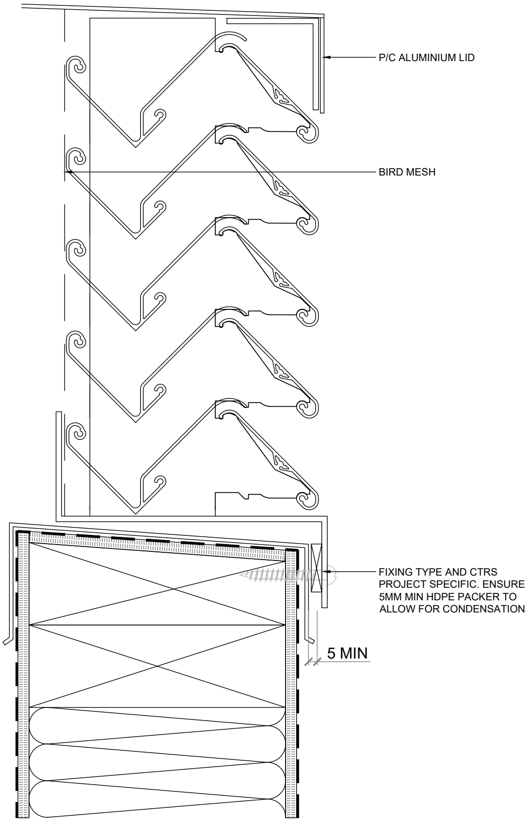
SECTION VIEW
