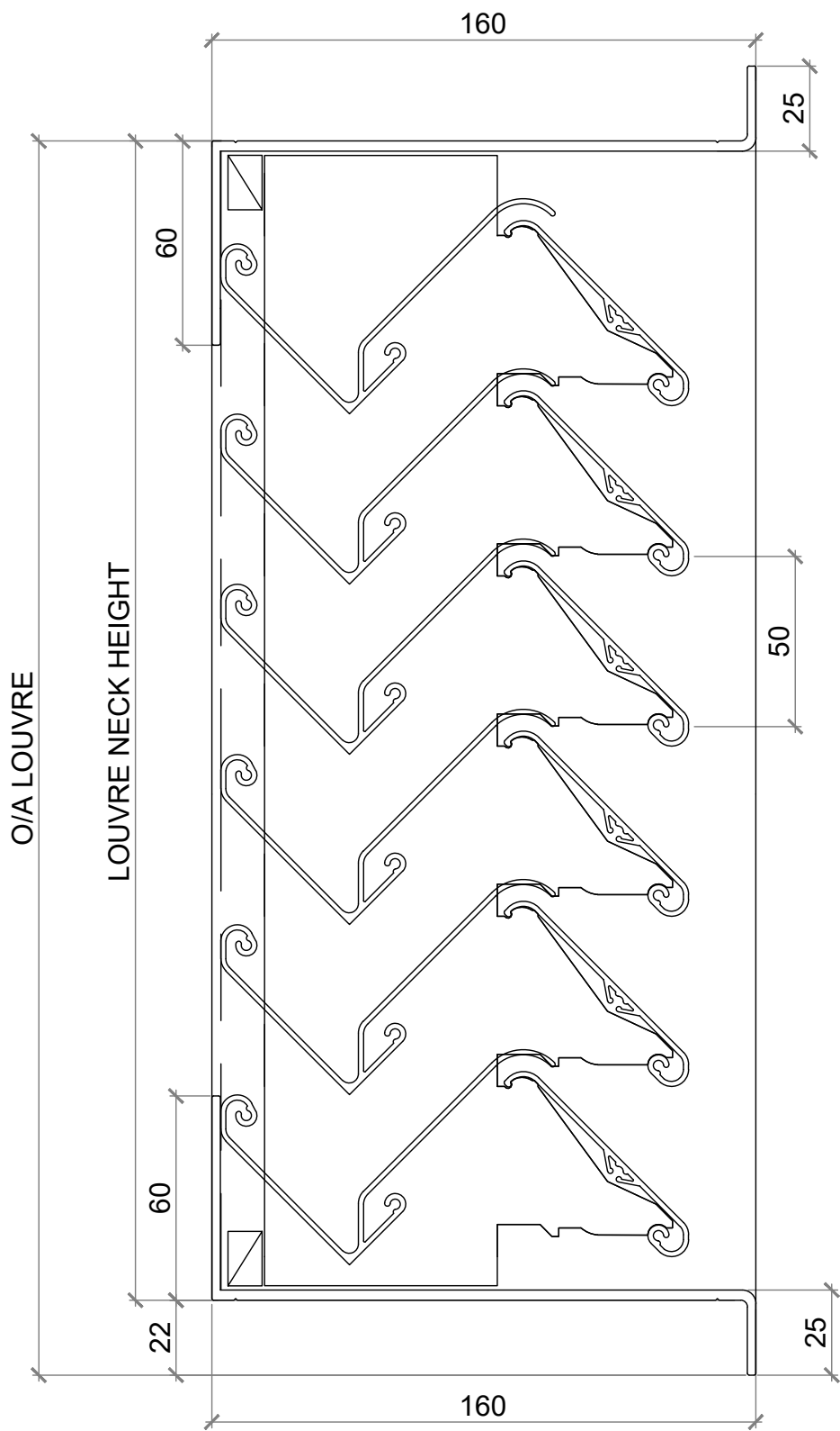
SECTION VIEW
