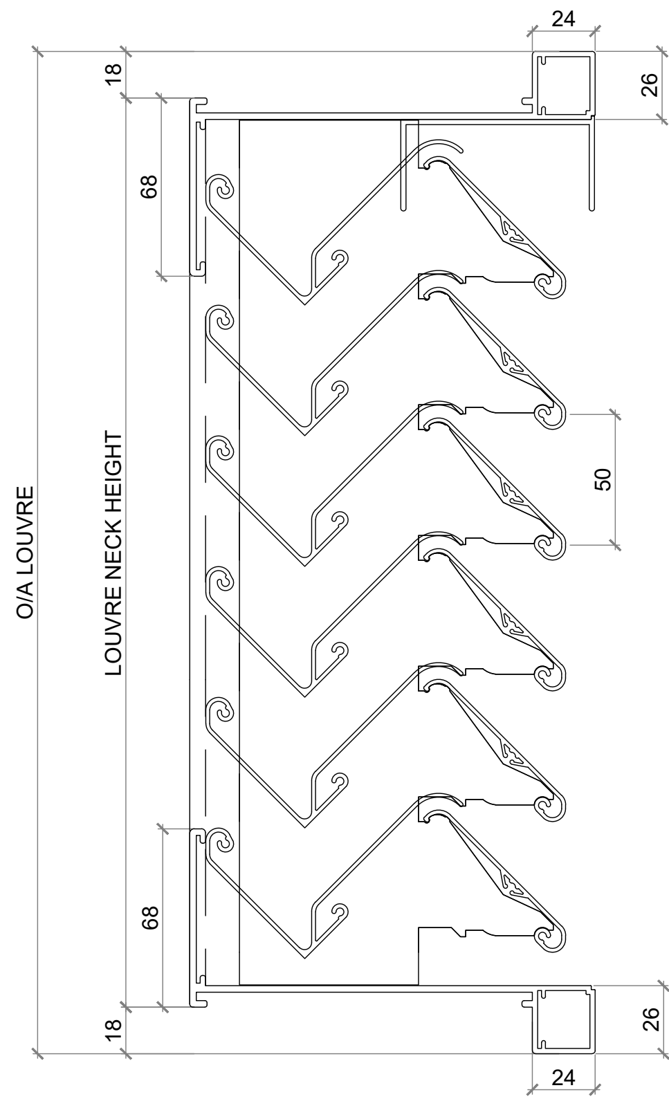
SECTION VIEW
