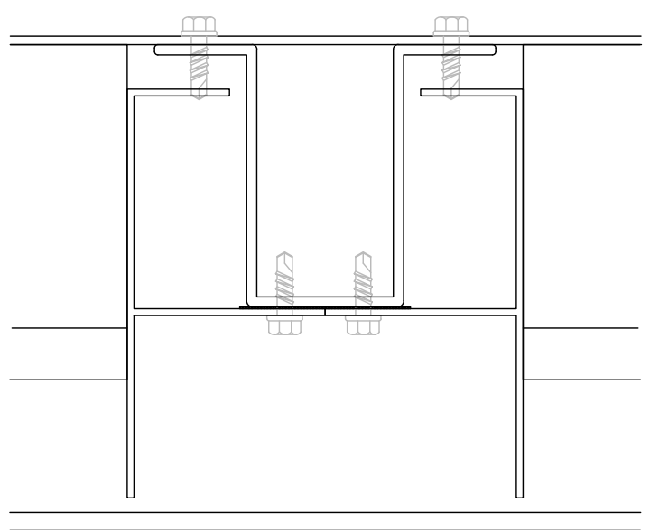
INTERMEDIATE MULLION REQUIRED FOR SPECIFIC LOADS
