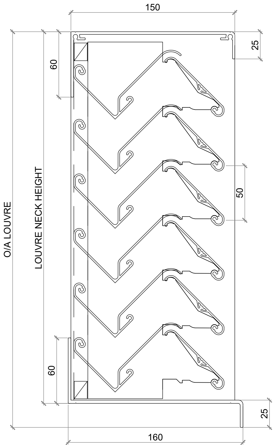
SECTION VIEW
