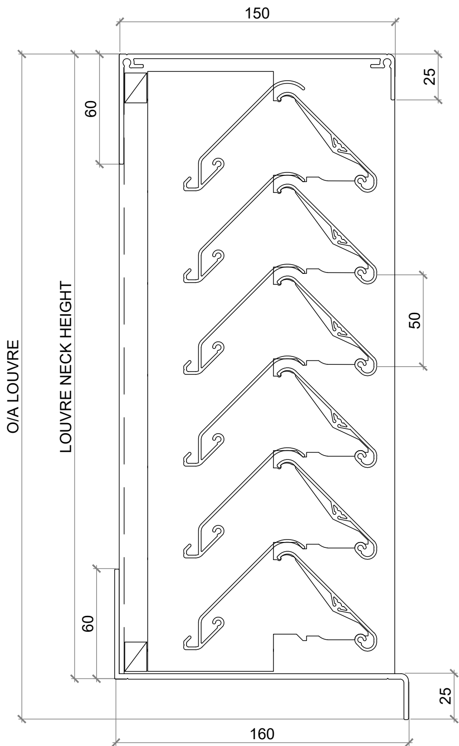
SECTION VIEW
