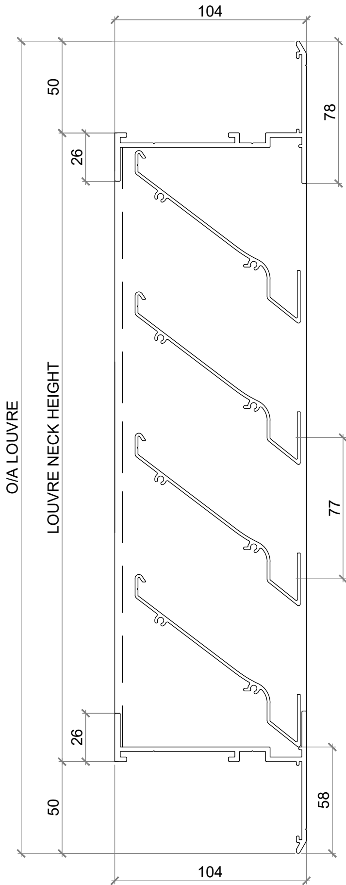
SECTION VIEW
