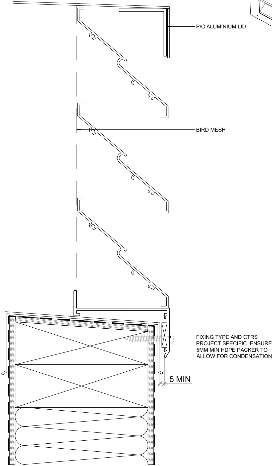
SECTION VIEW
