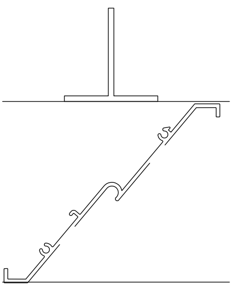
INTERMEDIATE STIFFENERS REQUIRED FOR SPECIFIC LOADS
