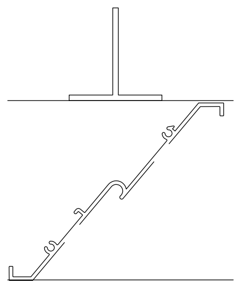
INTERMEDIATE STIFFENERS REQUIRED FOR SPECIFIC LOADS
