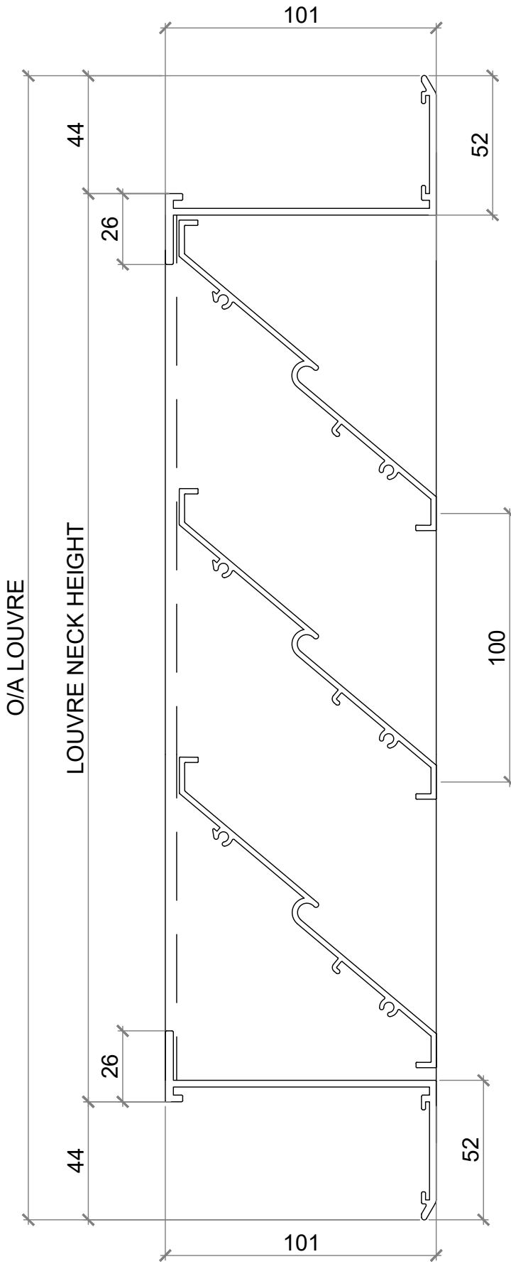
SECTION VIEW
