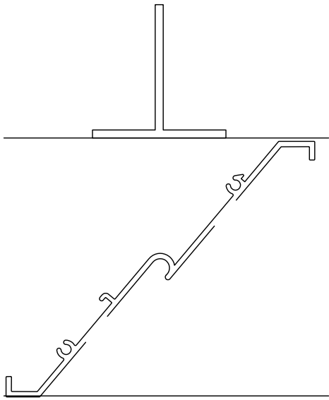
INTERMEDIATE STIFFENERS REQUIRED FOR SPECIFIC LOADS
