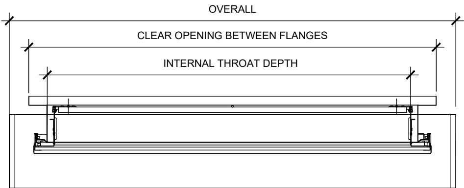
SECTION VIEW
