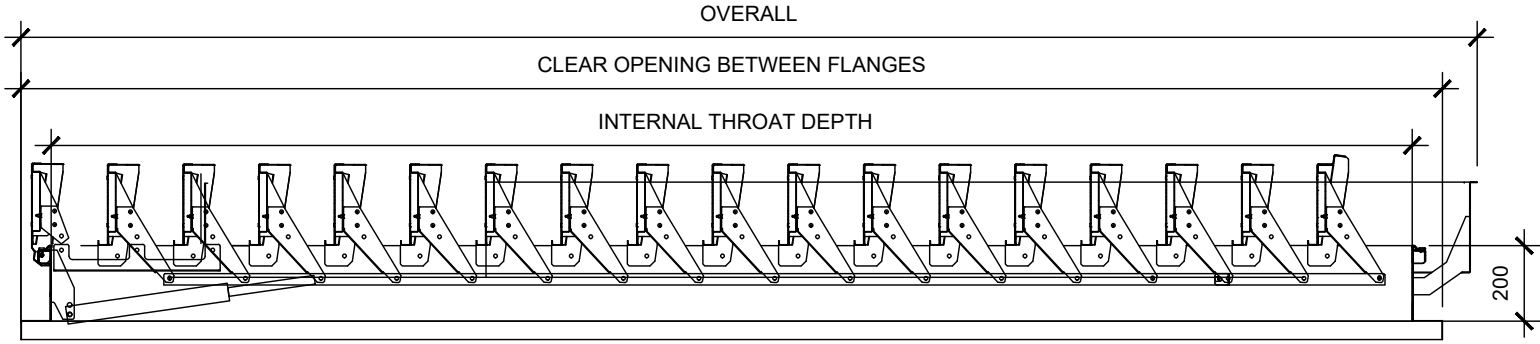
SECTION VIEW- OPEN
