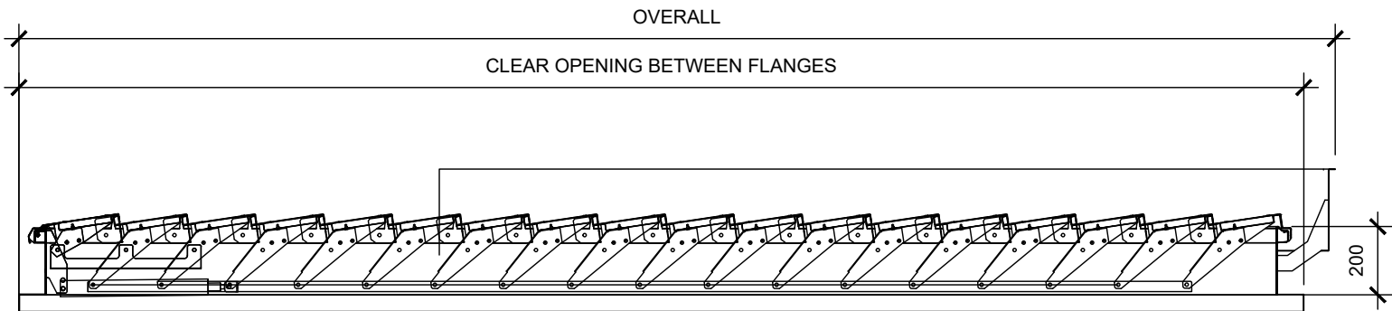
SECTION VIEW- CLOSED
