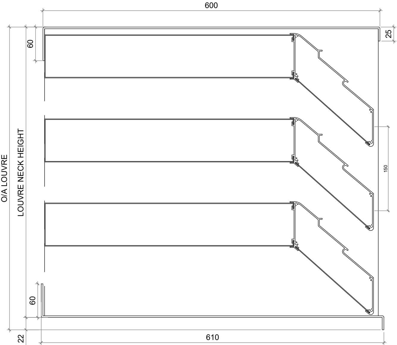
SECTION VIEW
