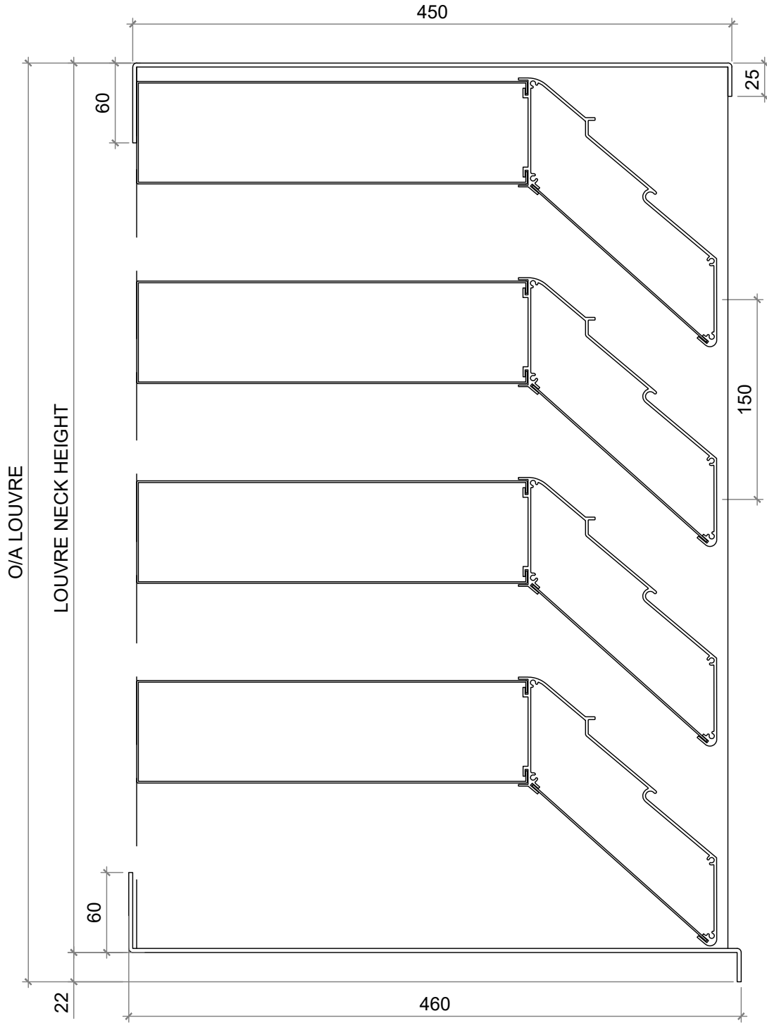
SECTION VIEW
