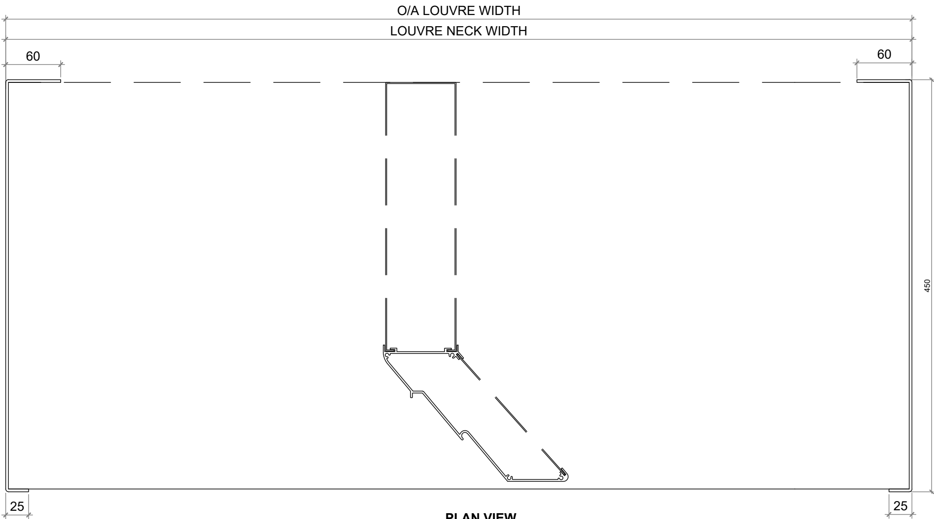
PLAN VIEW
