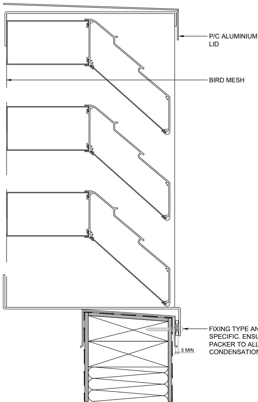
SECTION VIEW
