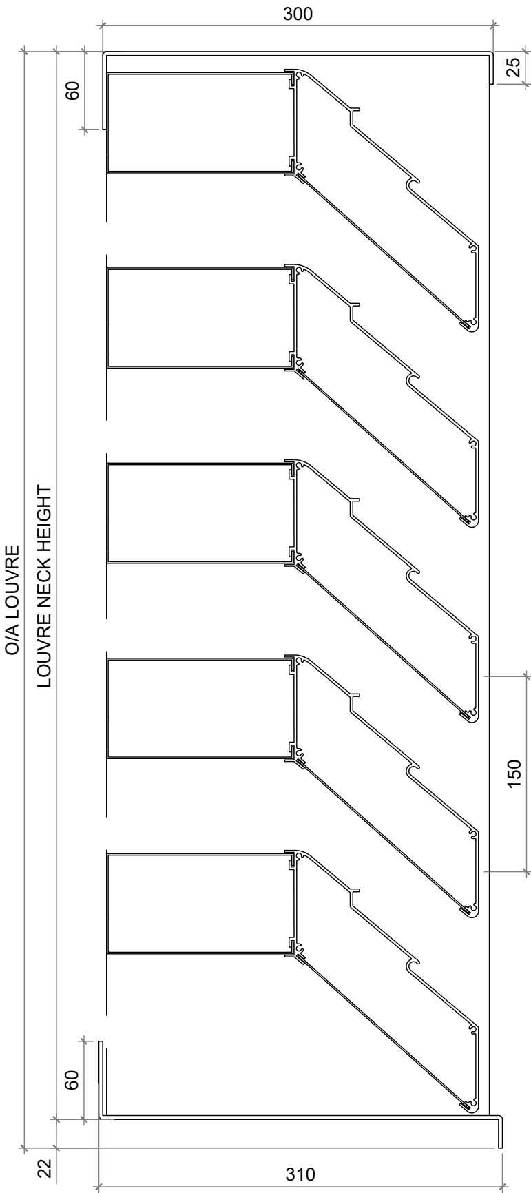
SECTION VIEW
