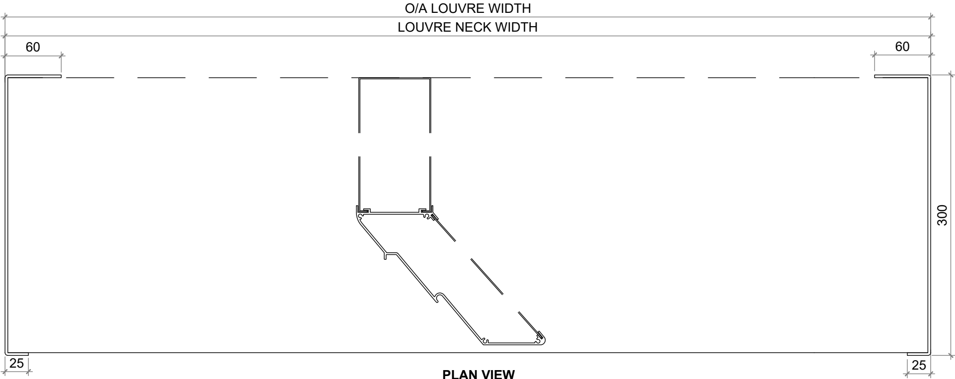
PLAN VIEW
