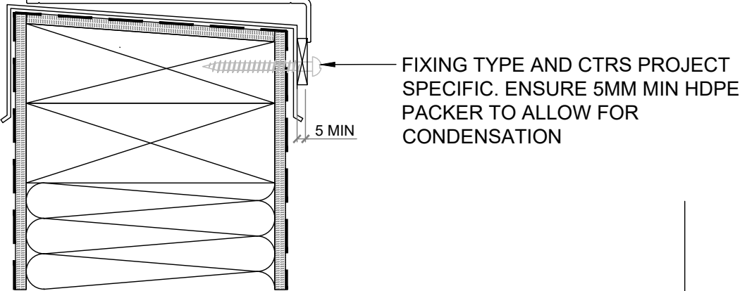
SECTION VIEW
