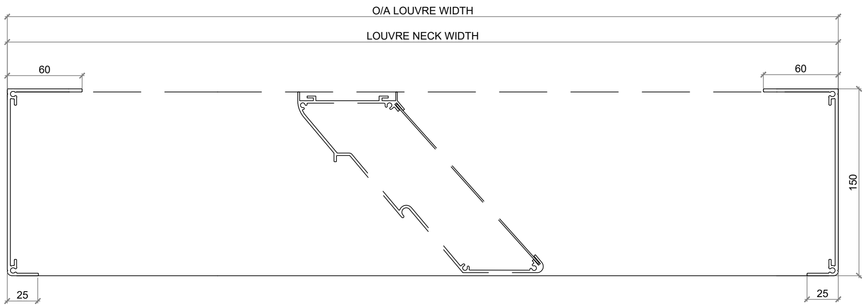
PLAN VIEW
