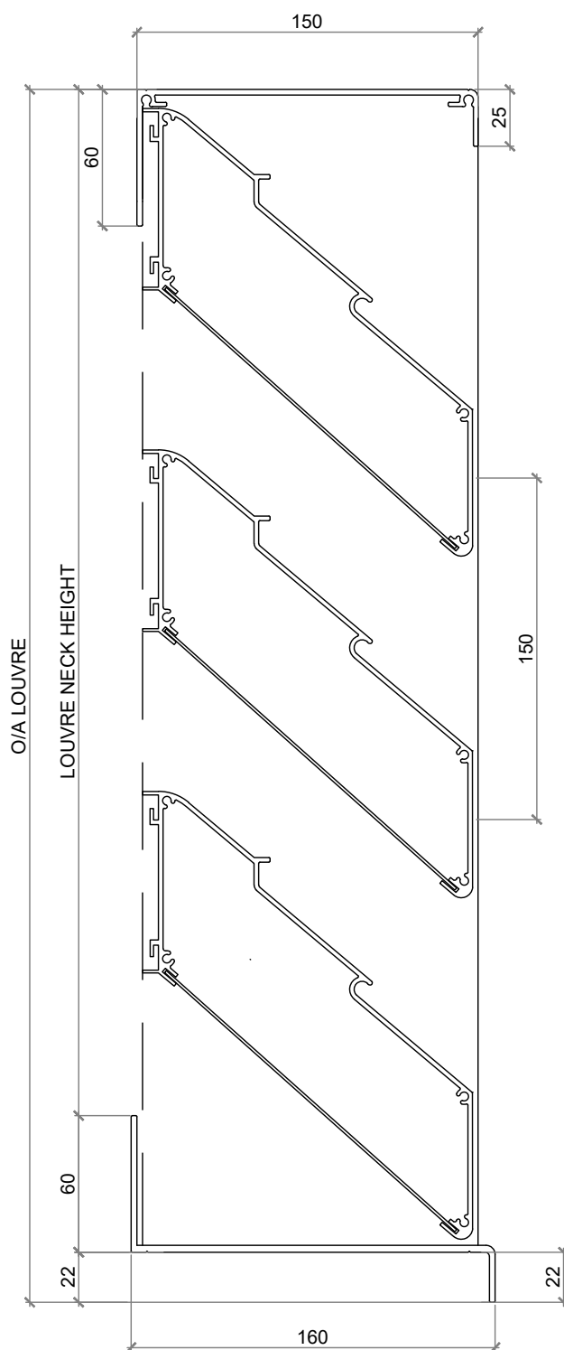
SECTION VIEW
