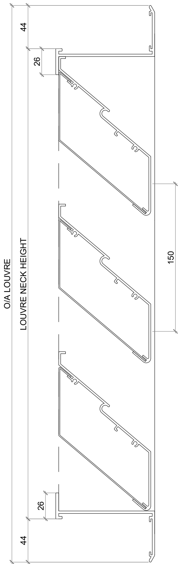
SECTION VIEW
